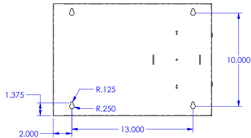
MOUNTING CONFIG
